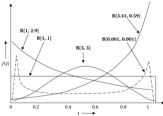
FIGURE 10.17 Beta distribution.
